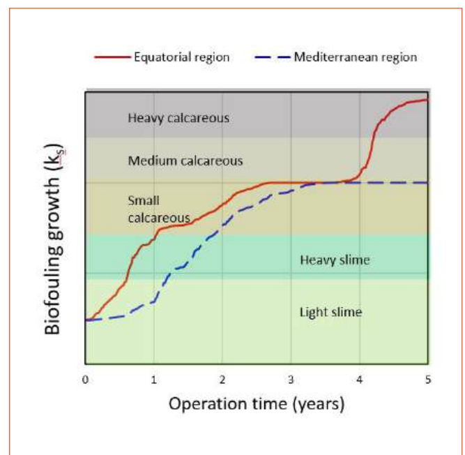
Figure 2 Biofouling growth on the hull under the No cleaning scenario in two different regions
